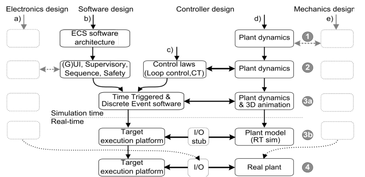
Figure 3. An overview of the design flow used for the SliderSetup [4], showing the different stages of the models and implementations.
